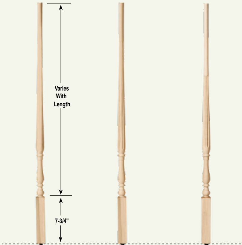
5715-P Plain 1-1/2 or 1-3/4" x 3X" 1-1/2 or 1-3/4" x 39" 1-1/2 or 1-3/4" x 41"
