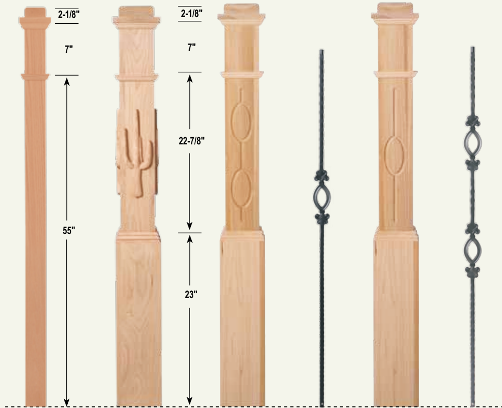
4075 62-1/8" BaseWidth: 3-1/2" Square
