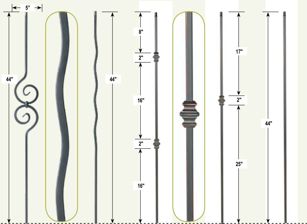
CS 2.10.1 Ends: 1/2" Ht: 44" Wt: 3.5 lbs. CS 2.2.3 Ends: 1/2" Ht: 44" Wt: 3 lbs. CS 16.1.35 Ends: 1/2" Ht: 44" Wt: 3 lbs. All Colors CS 16.1.34 Ends: 1/2" Ht: 44" Wt: 3 lbs. All Colors CS 16.2.1 Ends: 1/2" Ht: 44" Wt: 3 lbs. All Colors ← SAT B CV ORC ORB SP →
