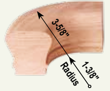
17 Radius Return End
