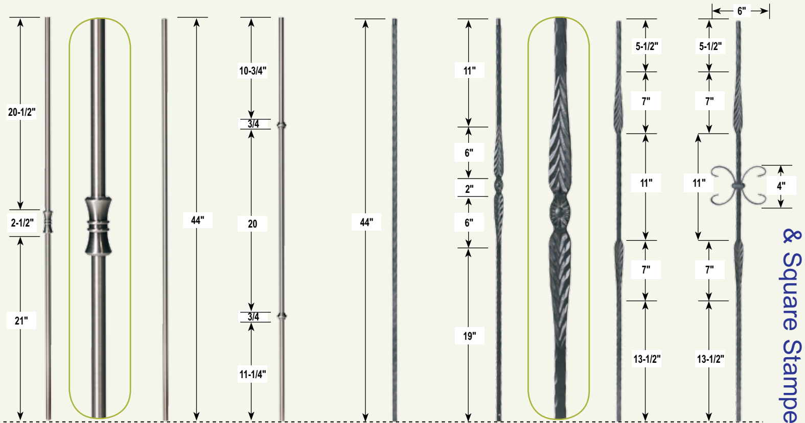
CS HG Ends: 5/8" Round Ht: 44" Wt: 3 lbs.
