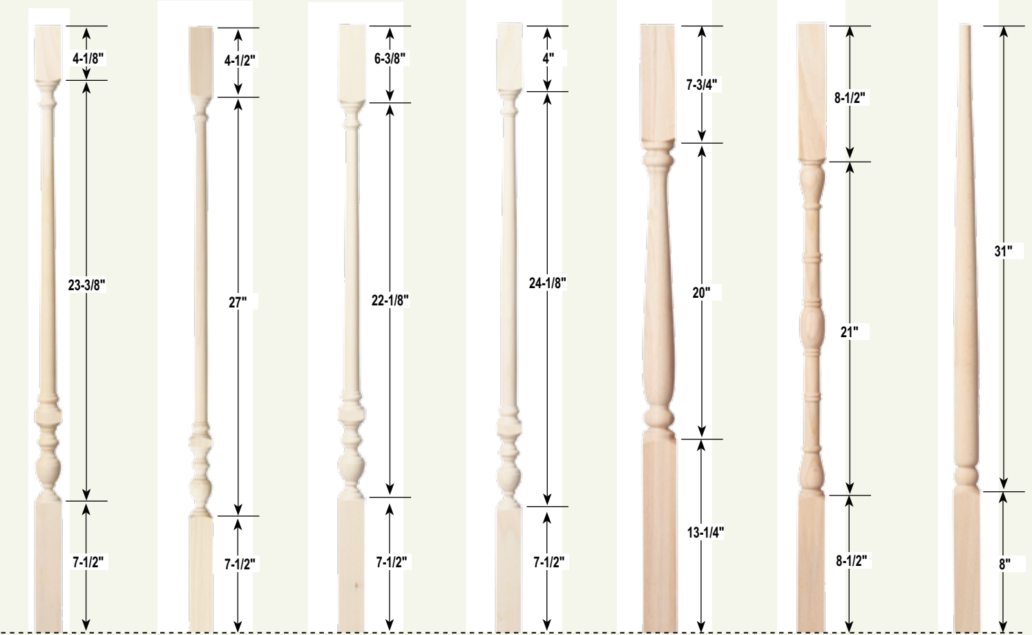
B-35 1-1/2" x 35" B-37 1-1/2" x 39" B-34 1-1/2" x 36" B-36 1-1/2" x 36" B-20 2-1/4" x 41" B-22 1-3/4" x 38" B-21 1-3/4" x 39"
