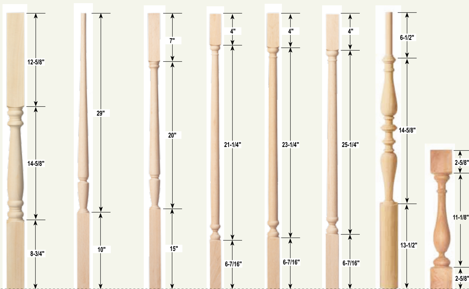
B-33 2-1/4" x 36" B-41 1-3/4" x 39" B-40 1-3/4" x 41" B-25 1-1/2" x 32" B-27 1-1/2" x 34-1/4" B-26 1-1/2" x 36" B-8 2-3/4" x 42" B-CIE-CV 2-5/8" x 16-1/4"
