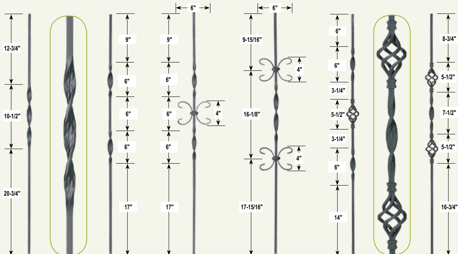
CS 16.1.5 Ends: 1/2" Ht: 44" Wt: 3.2 lbs. CS 16.1.6 Ends: 1/2" Ht: 44" Wt: 3.2 lbs. CS 16.1.10 Ends: 1/2" Ht: 44" Wt: 4 lbs. CS 16.1.11 Ends: 1/2" Ht: 44" Wt: 4 lbs. CS 16.3.6 Ends: 1/2" Ht: 44" Wt: 4 lbs. CS 16.3.7 Ends: 1/2" Ht: 44" Wt: 4 lbs.
