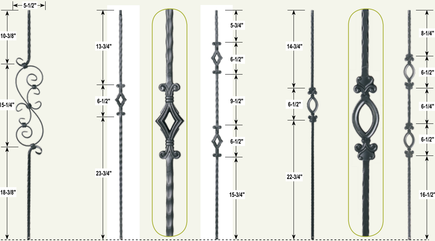
CS 2.9.7 Ends: 9/16" Ht: 44" Wt: 4 lbs. SAT ORB CS 2.9.3 Ends: 9/16" Ht: 44" Wt: 3.5 lbs. SAT B CV ORB CS 2.9.4 Ends: 9/16" Ht: 44" Wt: 3.8 lbs. SAT B CV ORB CS 2.9.5 Ends: 9/16" Ht: 44" Wt: 3.5 lbs. SAT B CV ORC ORB SP CS 2.9.6 Ends: 9/16" Ht: 44" Wt: 3.8 lbs. SAT B CV ORC ORB SP
