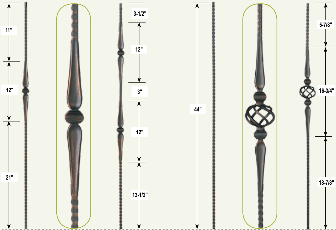
CS 16.5.2 Ends: 9/16" Square Ht: 44" Wt: 3.4 lbs. All Colors
