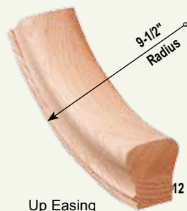
Up Easing
