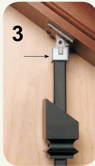
3 Snap Retaining Clip In Place
